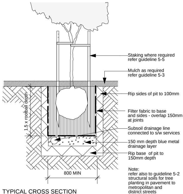
TYPICAL CROSS SECTION TREE PIT TO SOFT LANDSCAPED AREA (not to scale)
