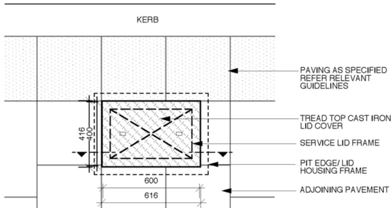
TYPICAL PLAN: STANDARD CAST IRON SERVICE LID COVER (not to scale)
