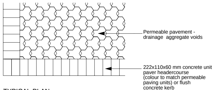
TYPICAL PLAN (not to scale)
