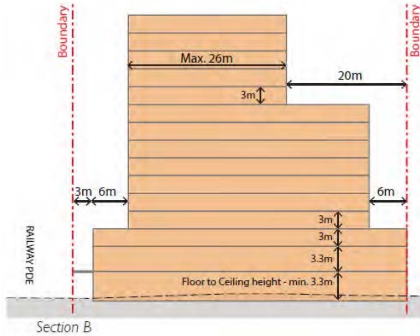
Figure 4.3.4.2.5 North-South Section of Site Building Envelope
