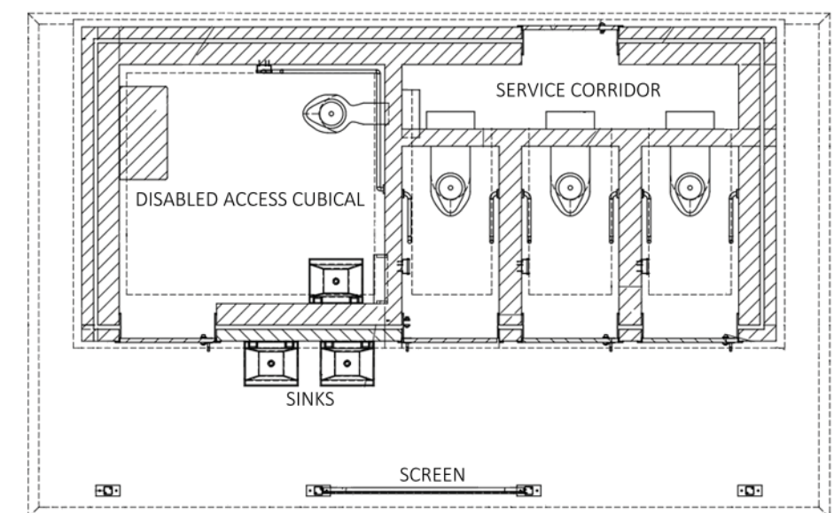
FLOOR PLAN OF PROPOSED AMENITIES BUILDING.
