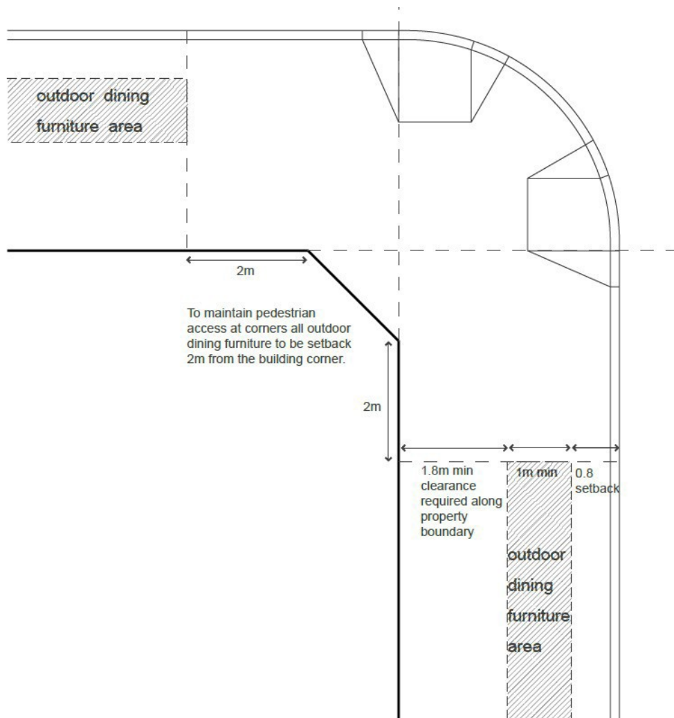
Diagram 4: Permissible layout at corners
