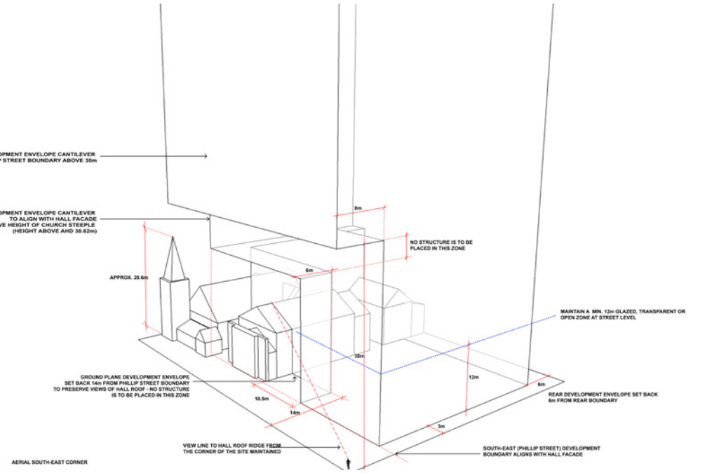
Figure 4.3.3.7.35 Maximum building envelope – Ground plane details, south west and south east corner elevations NTS (TKD Architects 2016)
