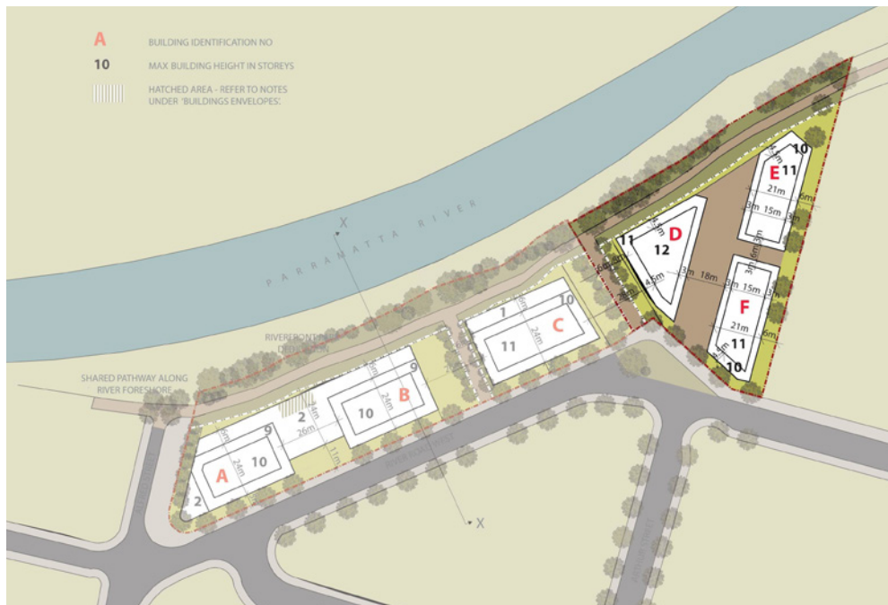
Figure 4.3.2.2.5 Building Envelopes
