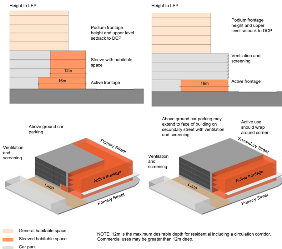
Figure 4.3.3.2 Frontage Treatments for Above Ground Car parking
