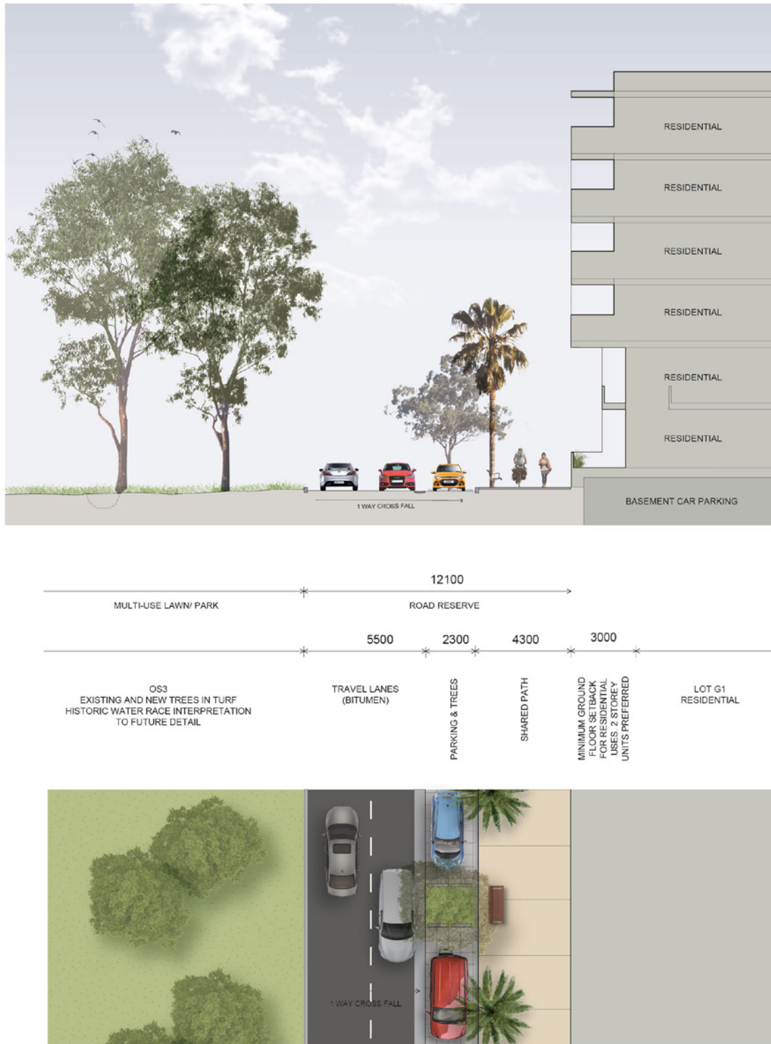
Figure 4.3.6.11 Typical street section 6 – East Circuit (east)
