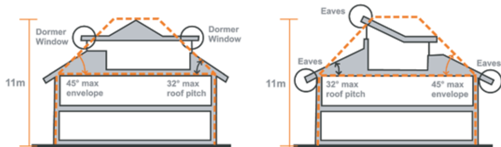
Figure 3.2.3.2 Roof envelope and pitch
