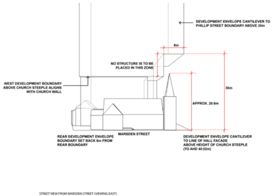
Figure 4.3.3.7.31 Maximum building envelope – Ground plane details, view from Marsden Street NTS (TKD Architects 2016)
