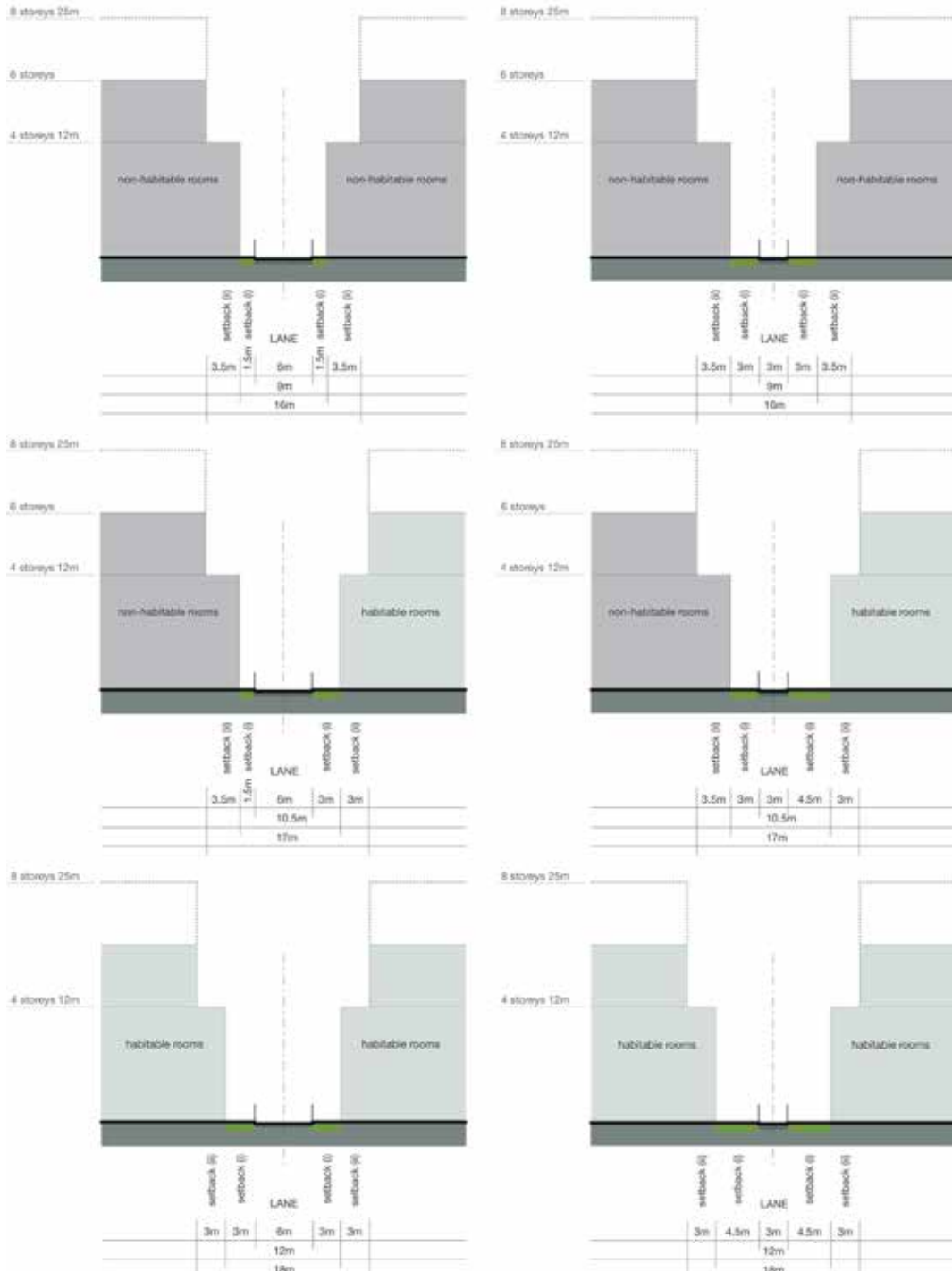
Figure 4.1.6.4 Lane and Street Sections
