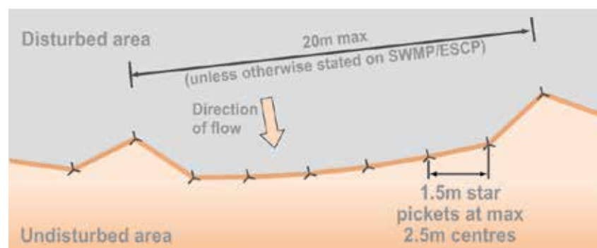
Figure 2.4.3.1.4 Plan - Sedimentation fencing Sources: Soils and Construction: Managing Urban Stormwater, Landcom, March 2004
