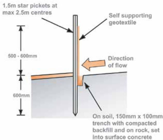
Figure 2.4.3.1.3 Section - Sedimentation fencing Sources: Soils and Construction: Managing Urban Stormwater, Landcom, March 2004
