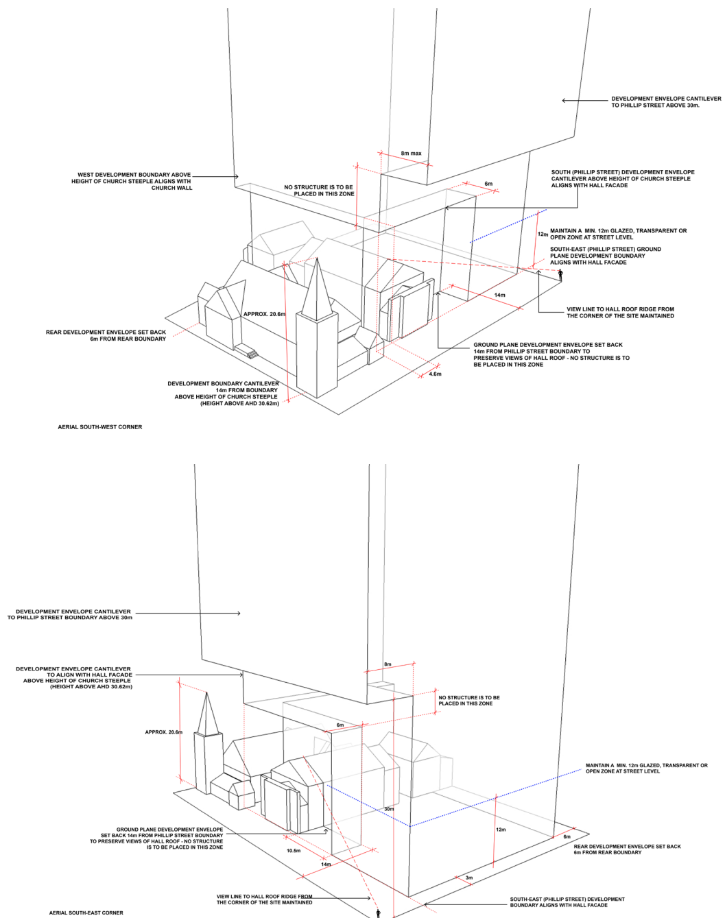
Figure 4.3.3.7.35 Maximum building envelope – Ground plane details, south west and south east corner elevations NTS (TKD Architects 2016)
