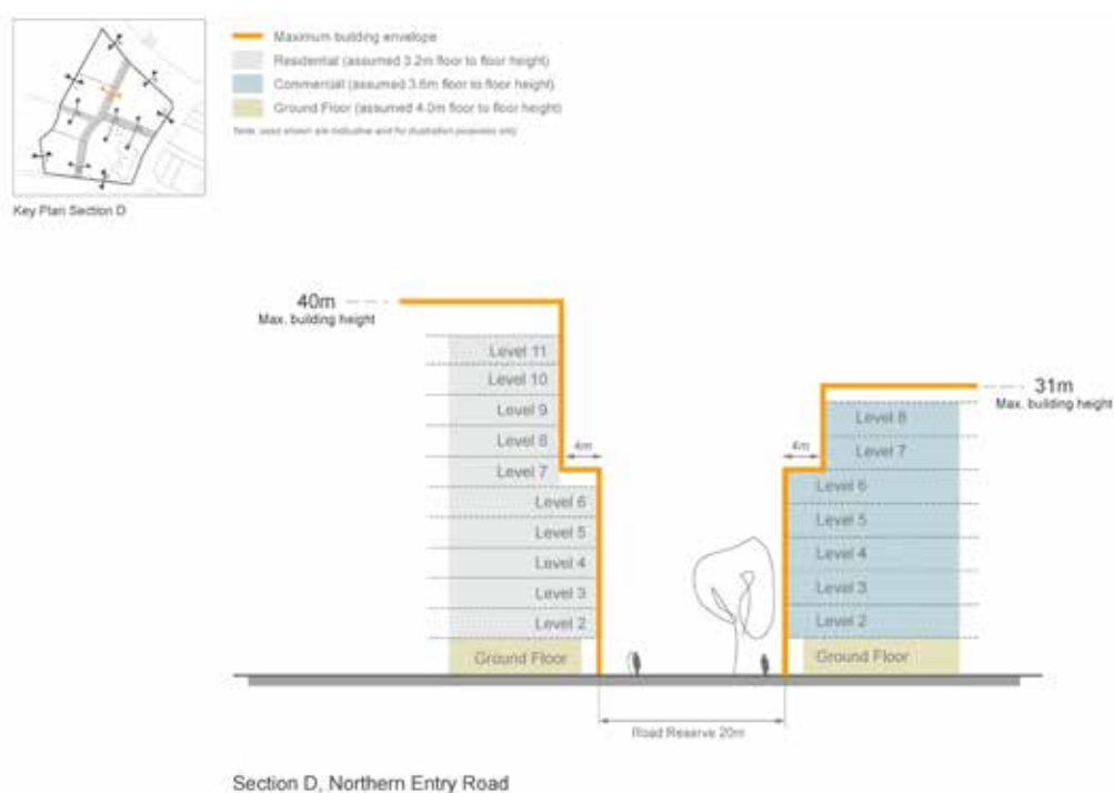
Figure 4.3.4.1.9 Indicative Site Sections
