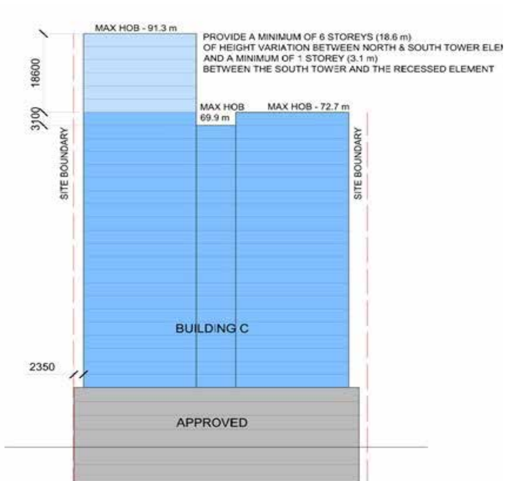
Figure 4.3.7.3.4 Elevation from Rowell Street
