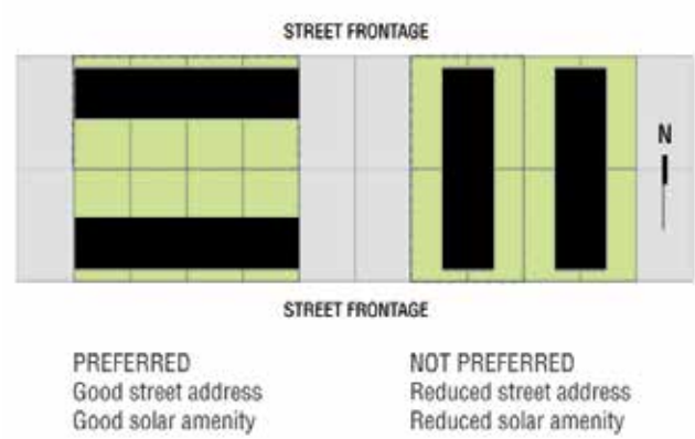
Figure 4.1.6.5 Preferred Street Frontage condition
