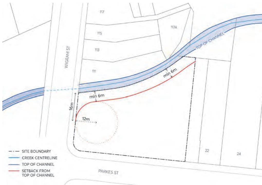
Figure 4.3.3.7.47 Required floodway setbacks for 14-20 Parkes Street
