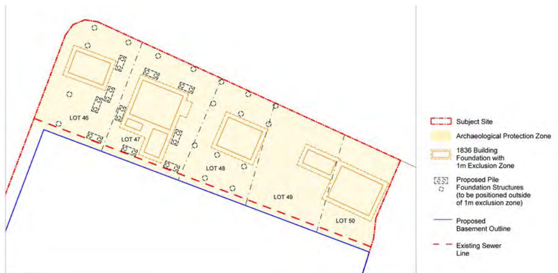
Figure 4.3.3.7.67 Control diagram: Piles and structures in relation to archaeological exclusion zone
