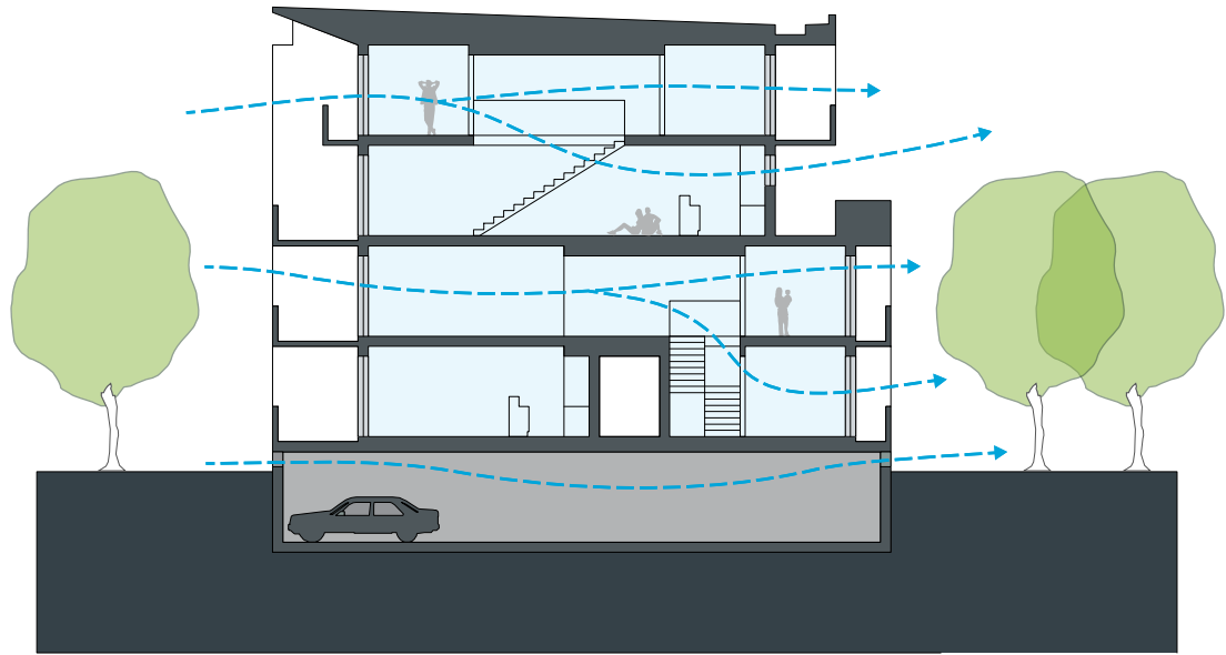
Figure 3.3.5.5 Cross ventilation of apartments Source: Apartment Design Guide, Department of Planning & Environment
