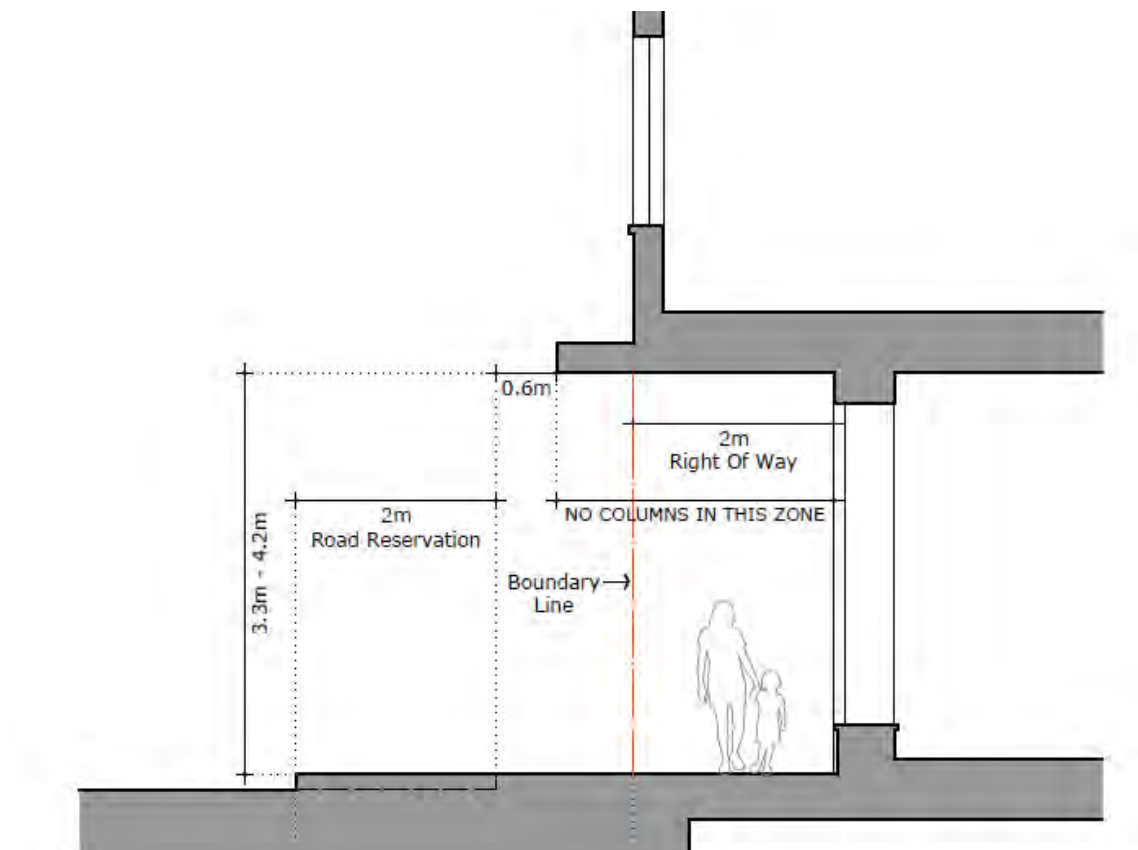
Figure 4.3.3.7.82 Detailed Section through Marsden Street
