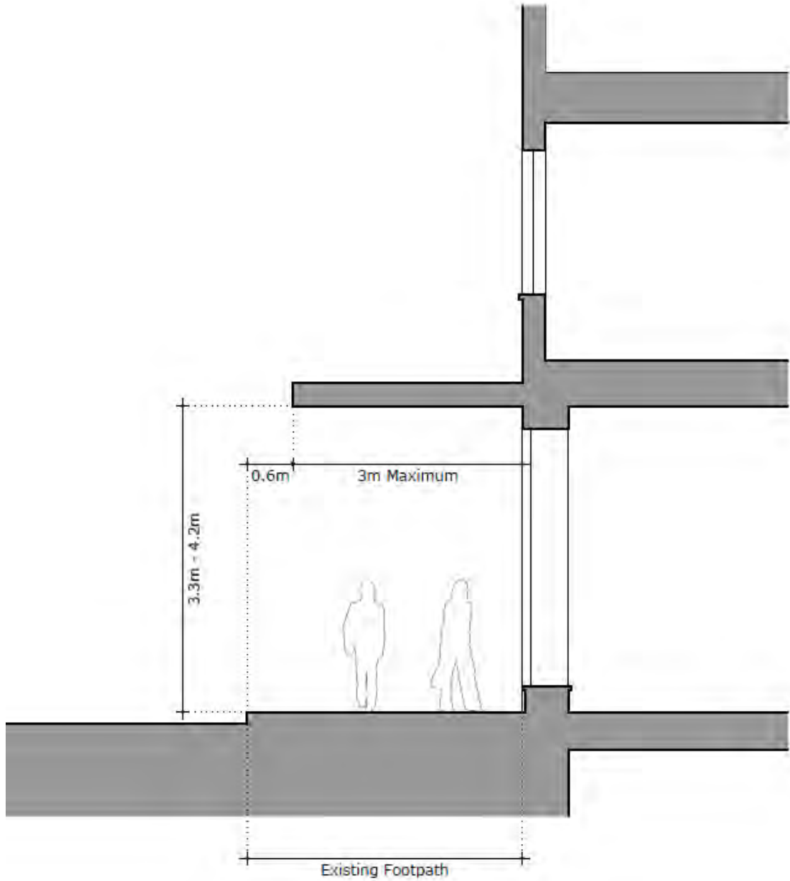
Figure 4.3.3.7.80 Detailed Section through Macquarie Street
