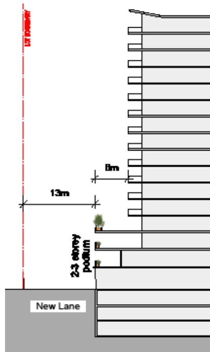
Figure 4.1.5.11 Setbacks to New Lane connecting Carlingford Road and Rawson Street
