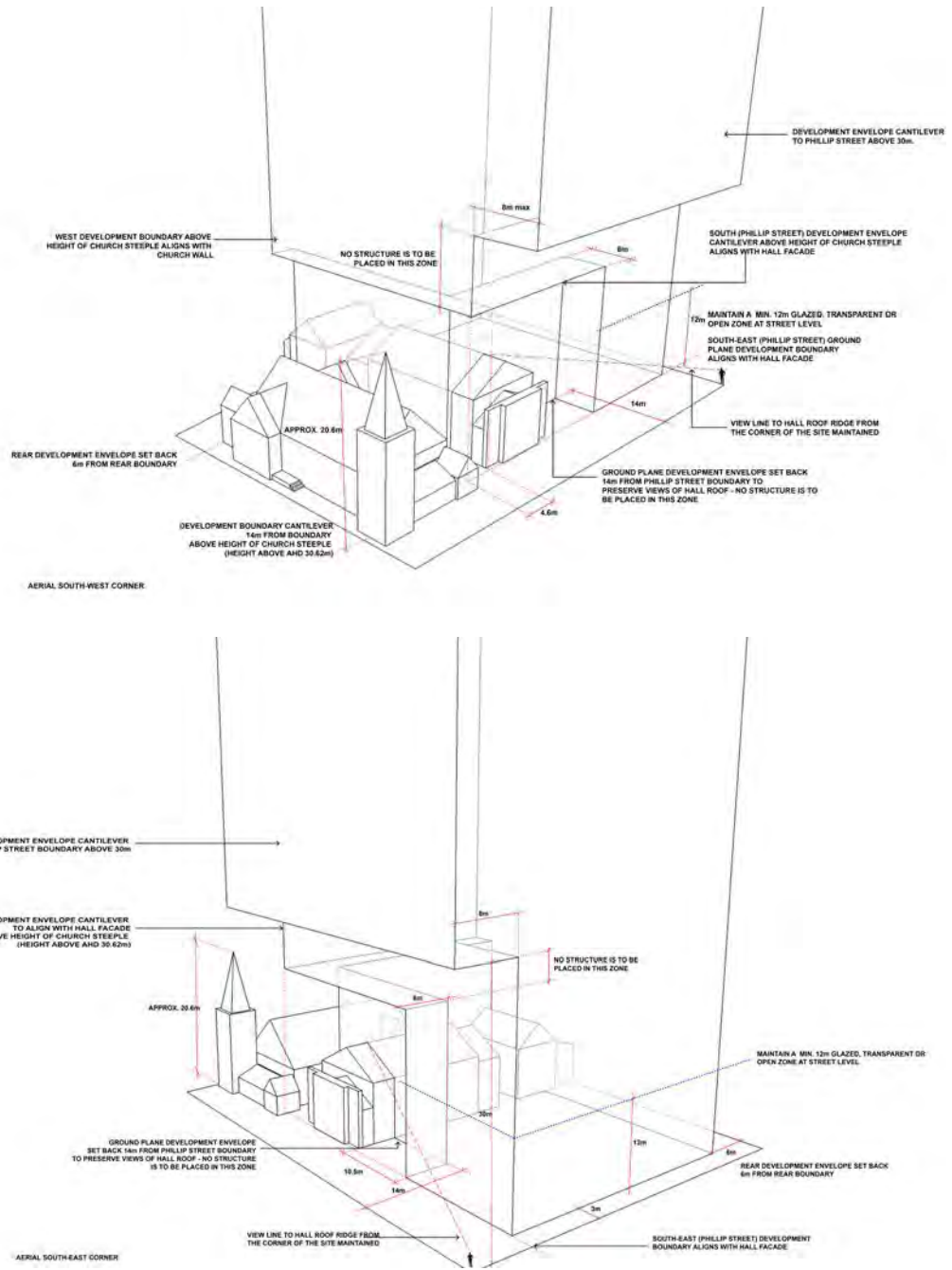
Figure 4.3.3.7.35 Maximum building envelope – Ground plane details, south west and south east corner elevations NTS (TKD Architects 2016)
