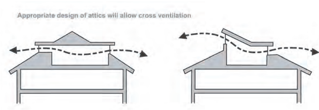
Figure 3.3.5.3 Attic design to enhance cross ventilation
