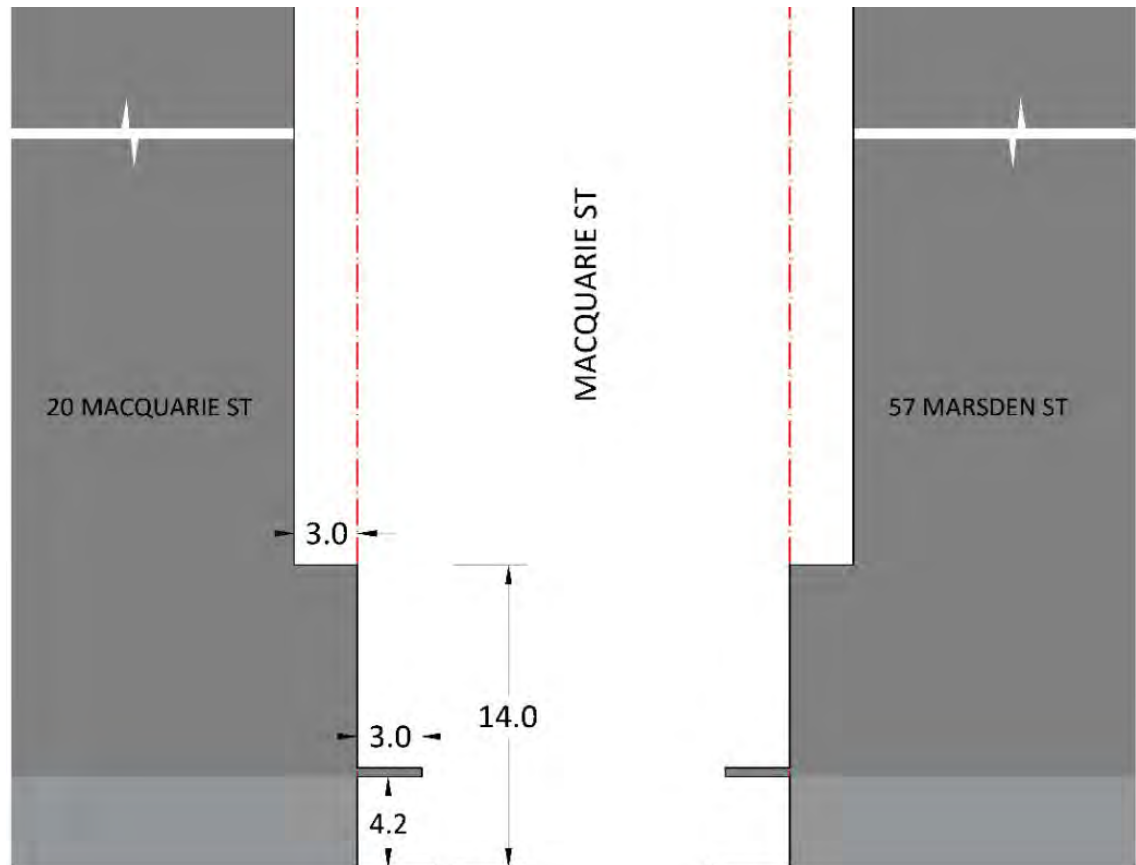
Figure 4.3.3.7.79 Section 1 through Macquarie Street
