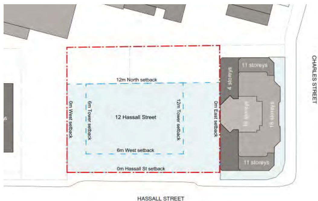
Figure 4.3.3.7.75 Built form – setback and tower separations.
