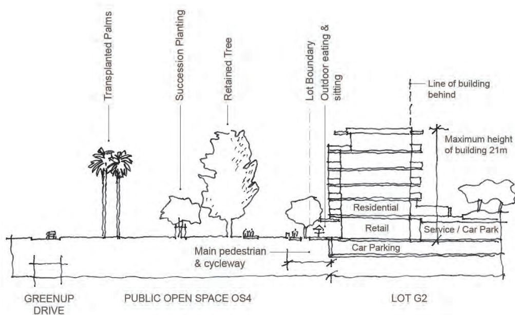
Figure 4.3.6.39 Lot G2 interface with open space
