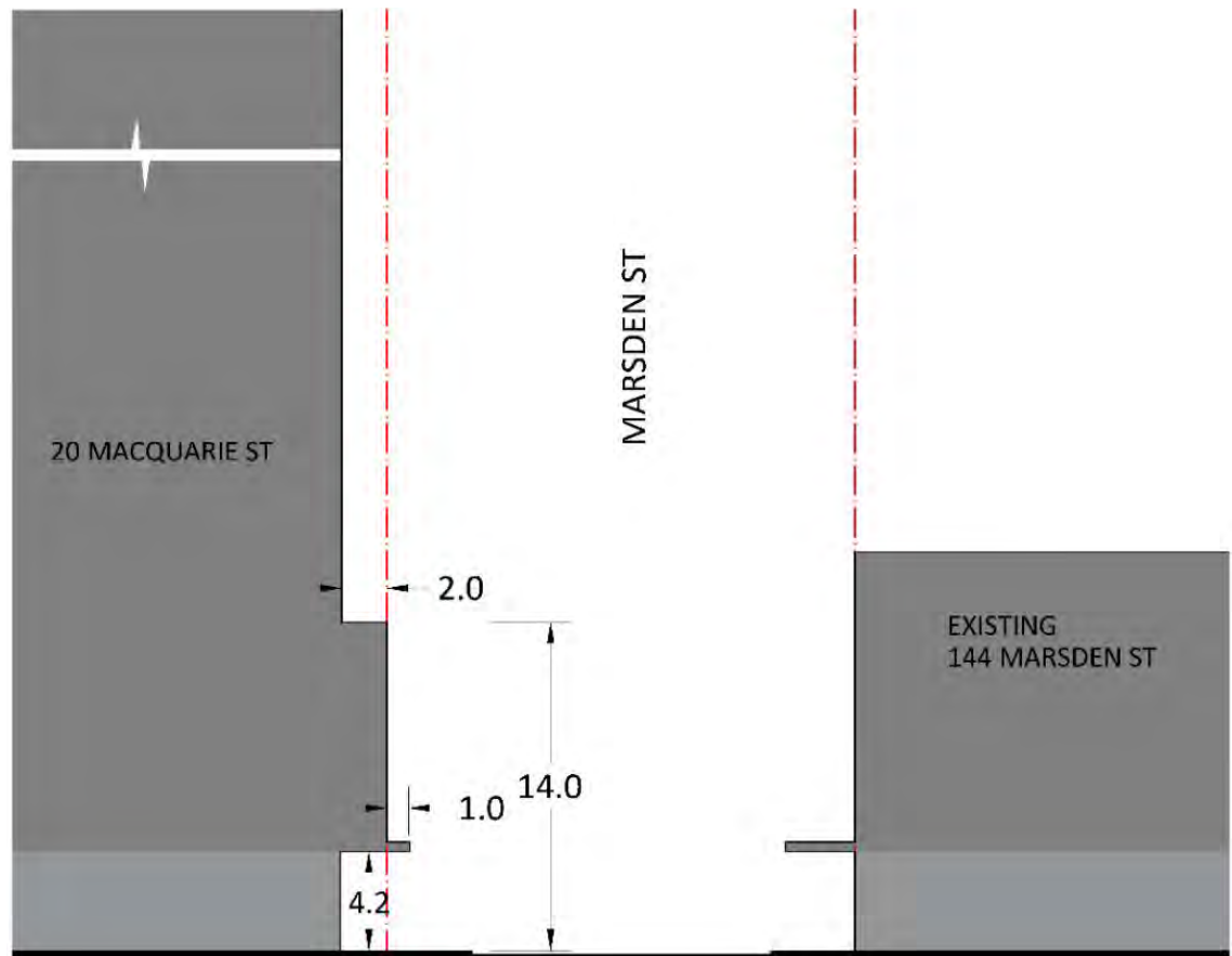
Figure 4.3.3.7.81 Section 2 through Marsden Street
