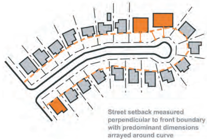
Figure 3.2.5.3 Building frontage setbacks - curvilinear street
