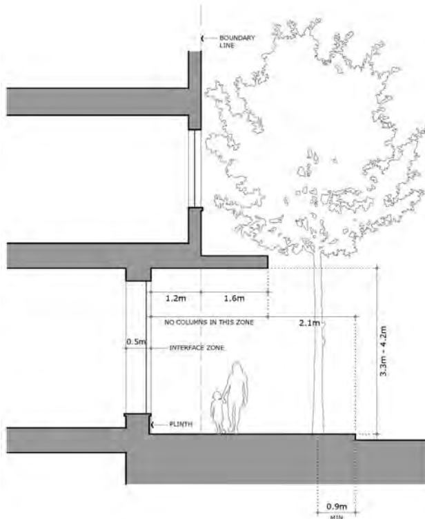
Figure 4.3.3.7.73 Street Section Aird St, O'Connell St and Campbell St
