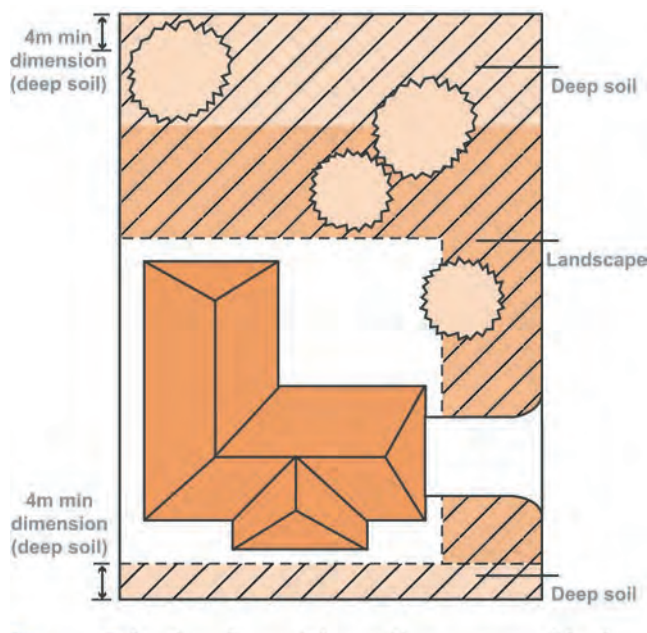
Figure 3.3.1.3 Landscaping and deep soil zones as combined feature of site design
