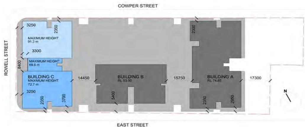
Figure 4.3.7.3.2 Building C Envelope, Heights and Setbacks
