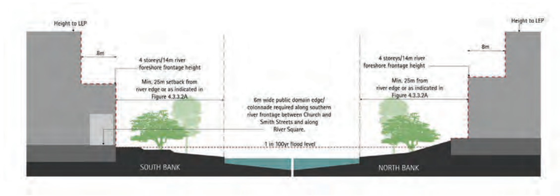
Figure 4.3.3.1.8 River Frontage Heights and Upper Level Setbacks River Foreshore
