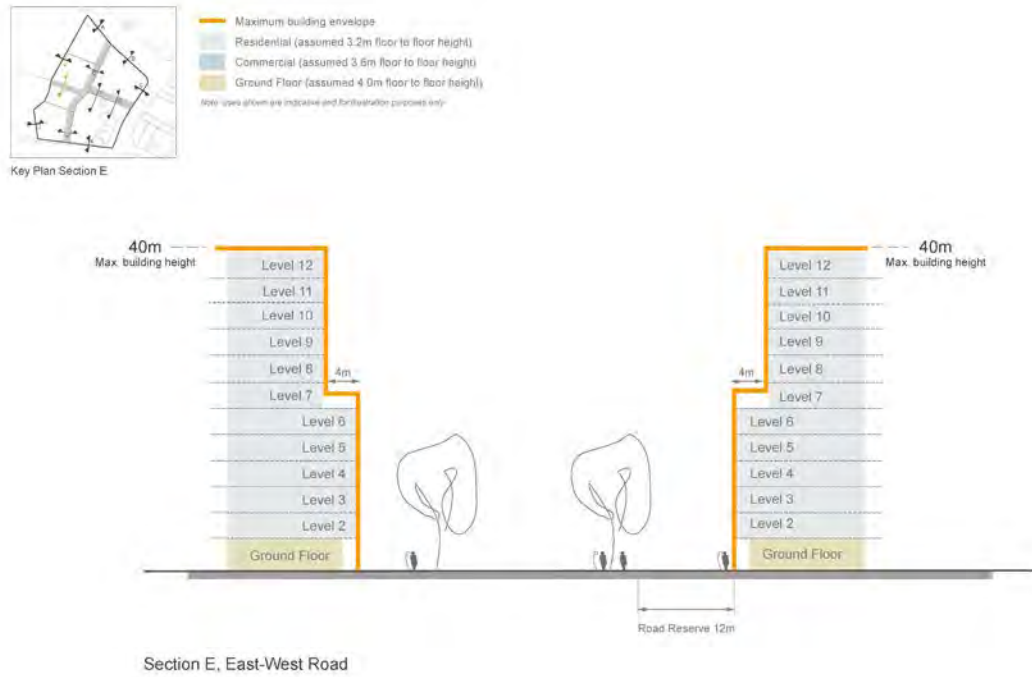
Figure 4.3.4.1.10 Indicative Site Sections
