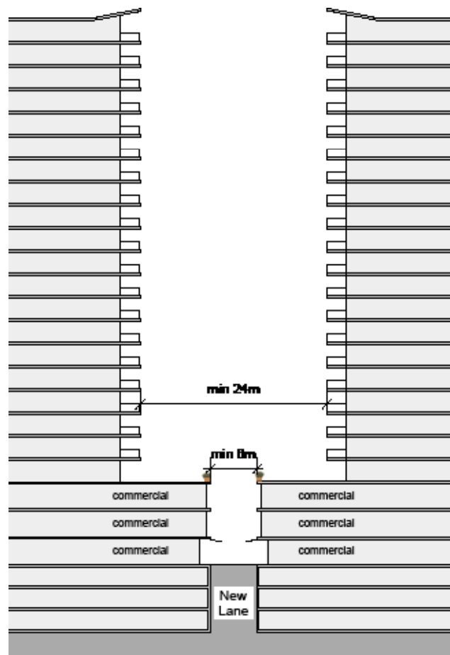
Figure 4.1.5.12 Setbacks to New Lane connecting Rawson Street to Becroft Road
