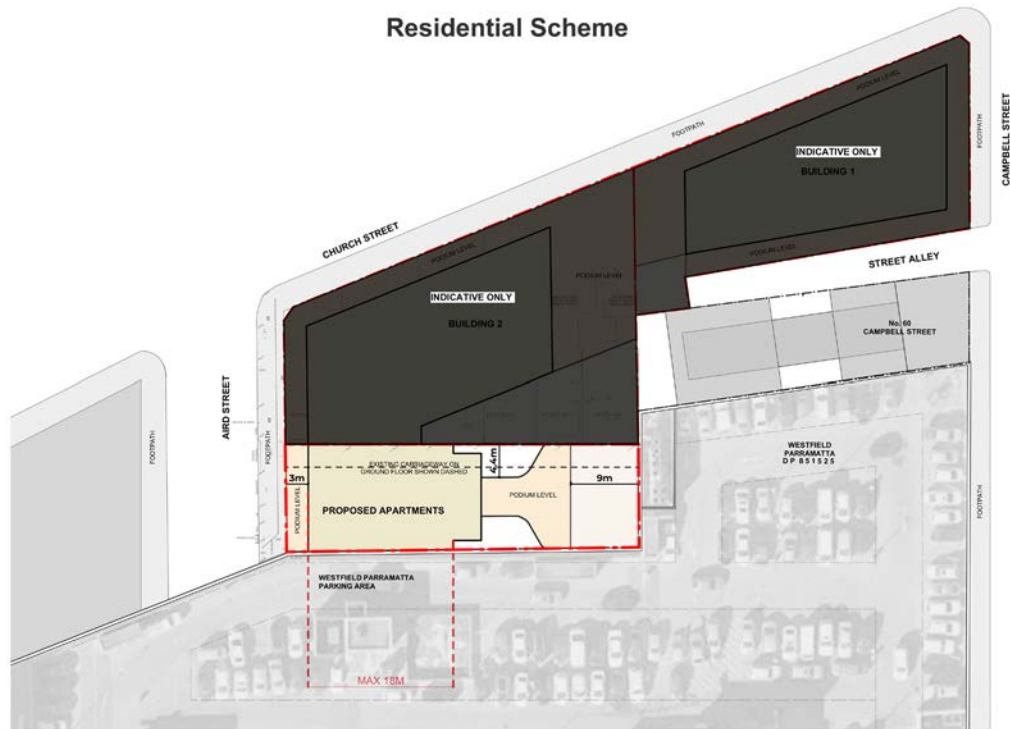
Figure 4.3.3.7.49 Residential Scheme Building Envelope
