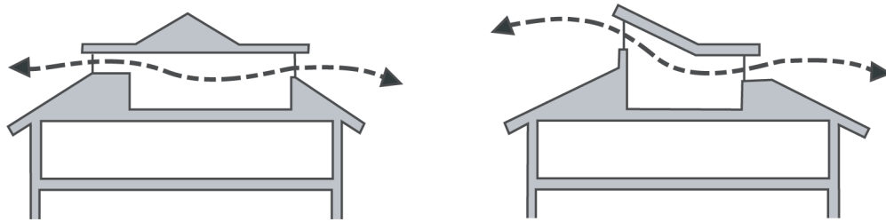
Figure 3.3.5.3 Attic design to enhance cross ventilation
