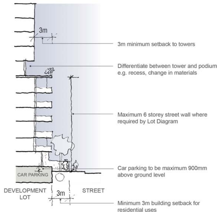
Figure 4.3.6.21 Typical Street wall heights and tower setbacks
