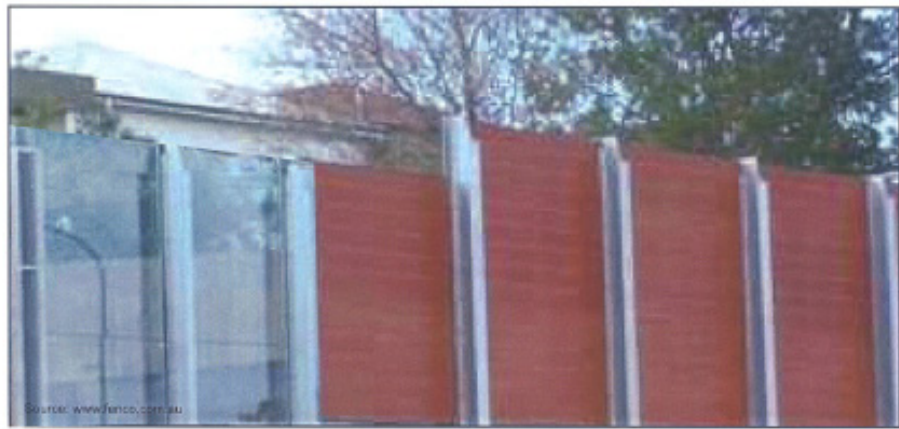
Examples of acoustic barrier designs for sloping sites where an effective height of up to 4 m is required
