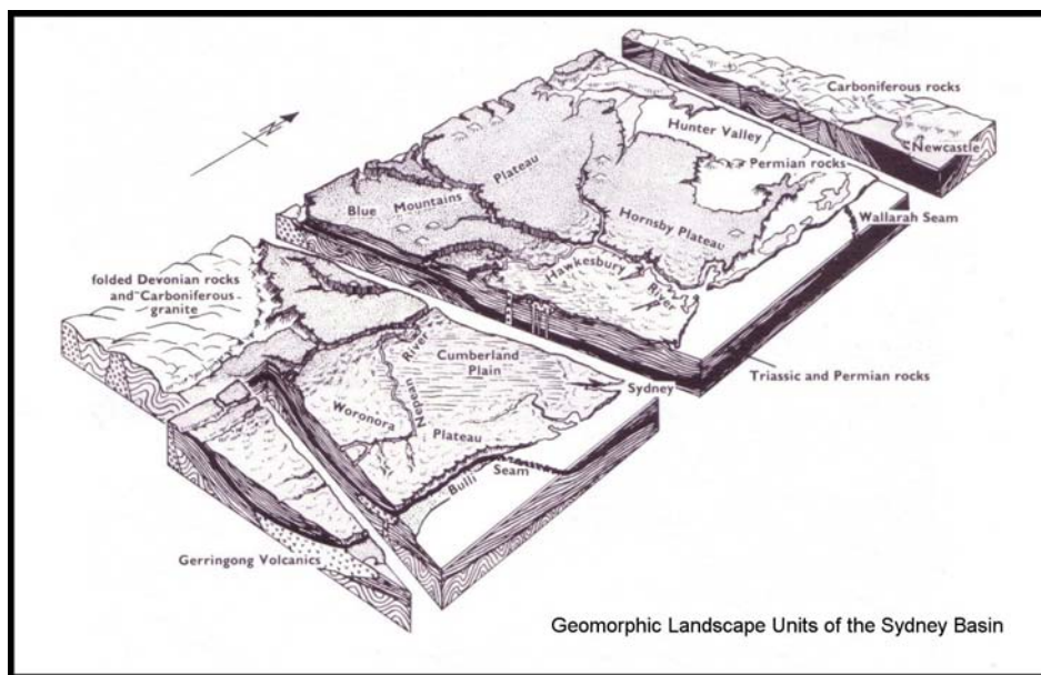
Figure 3. Geomorphologic landscape units of the Sydney Basin. (Source: Branagan et al. 1976; Herbert and Helby 1980)
