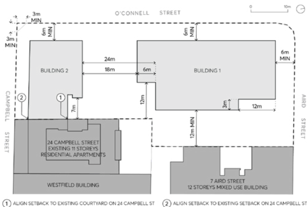
Figure 6.10.12.1 – Building Envelopes
