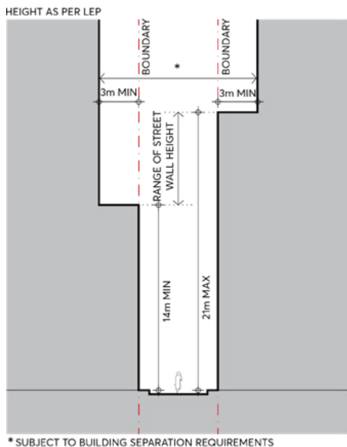
Figure 6.3.3.1.4 – Laneway Setbacks
