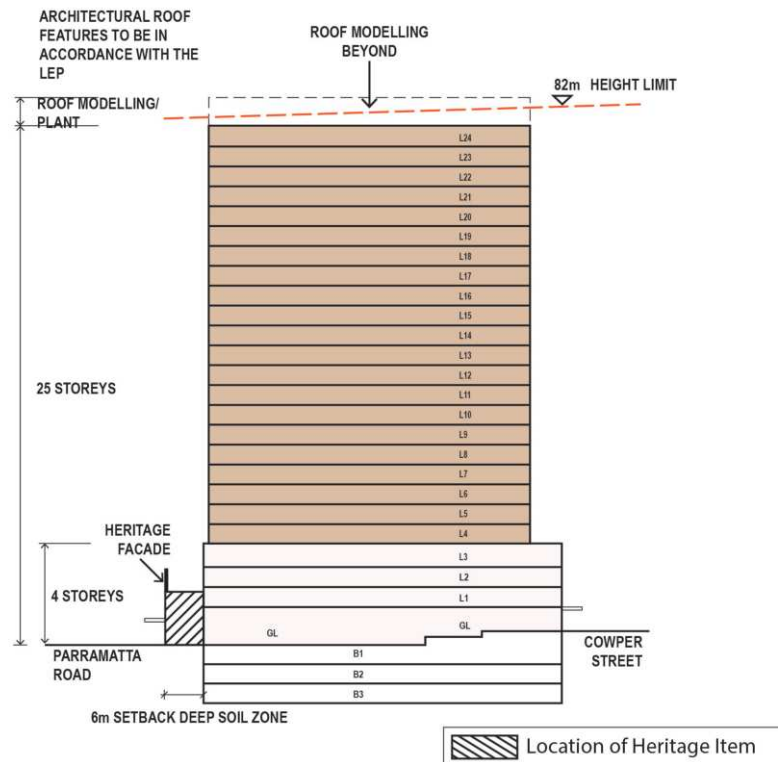
Figure 8.5.3.4.3 - Building envelope section B-B
