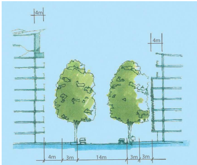
Figure 8.3.4.1.5 - Type E tower element building as viewed from Morton Street looking north
