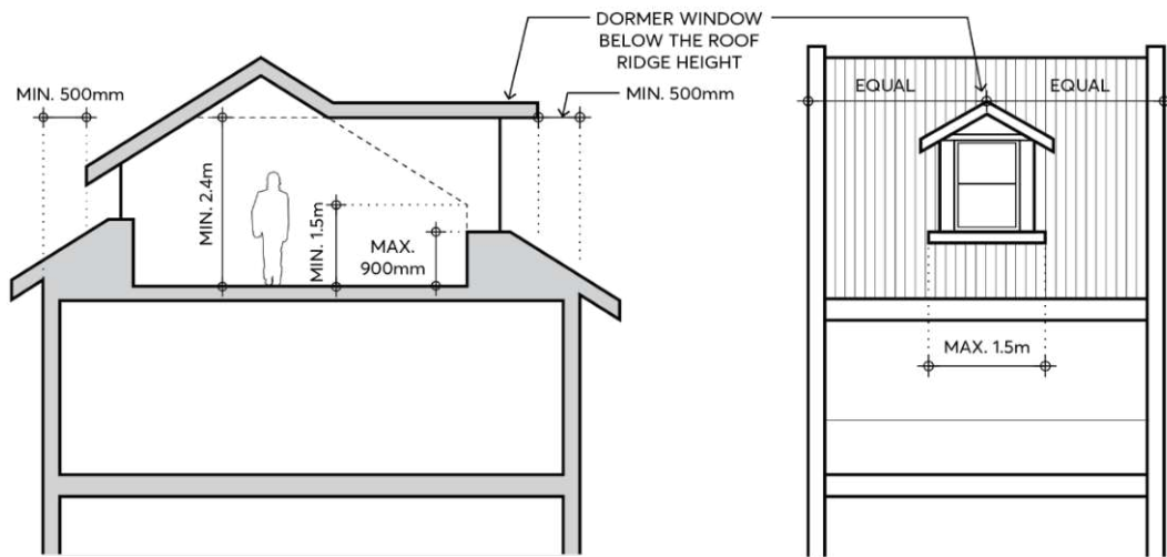
Figure 3.2.3.1 – Attic design
