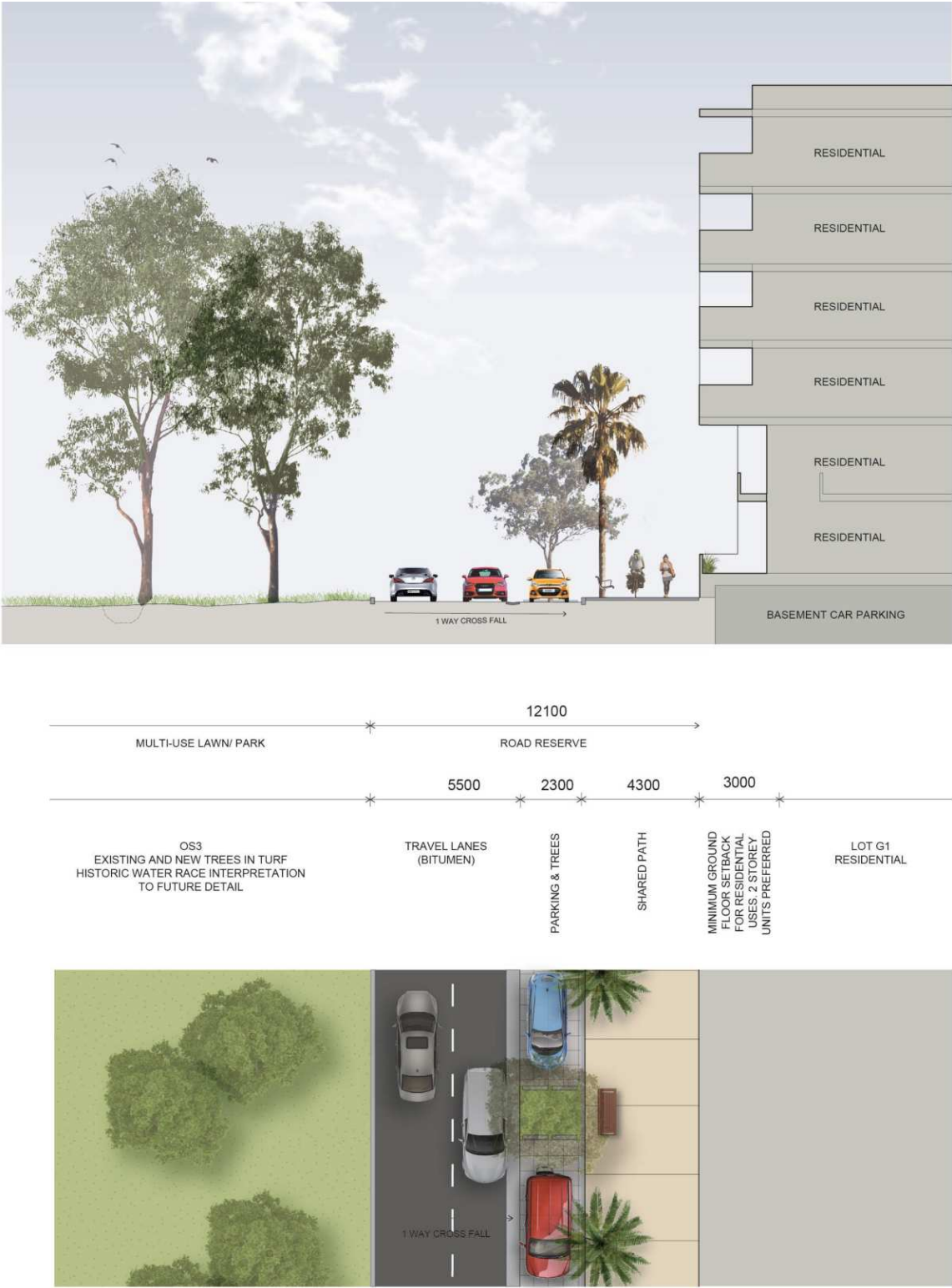
Figure 8.2.2.6.6 - Typical street section 6 – East Circuit (east)
