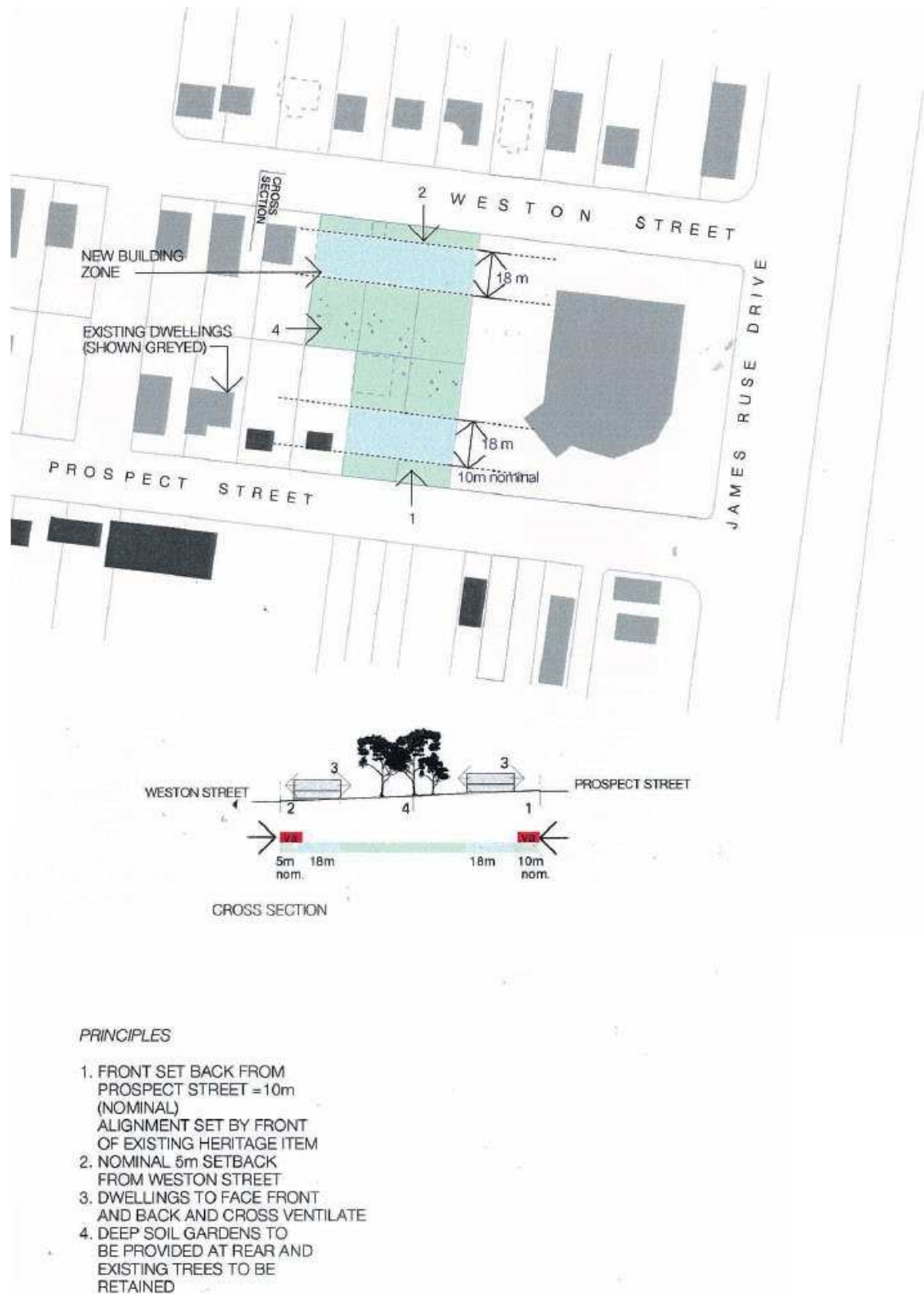
Figure 8.3.2.6.2 – Key Block 7
