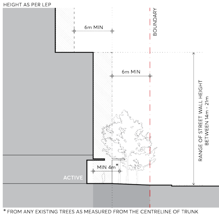
Figure 9.5.6.5 – Great Western Highway (Section C) Setbacks and Street Wall Height
