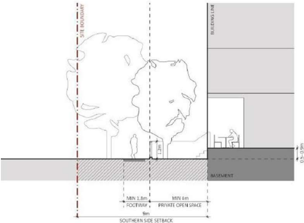
Figure 8.5.10.2.5 – Southern Setback Condition
