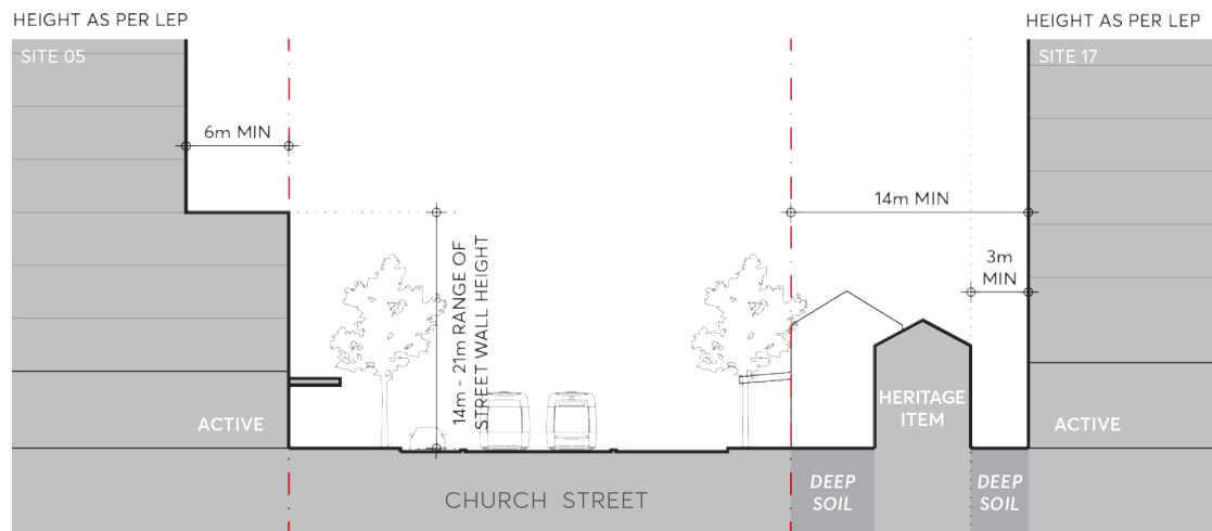
Figure 9.5.11.13 – Site 17 (Section I) Setbacks and Street Wall Height
