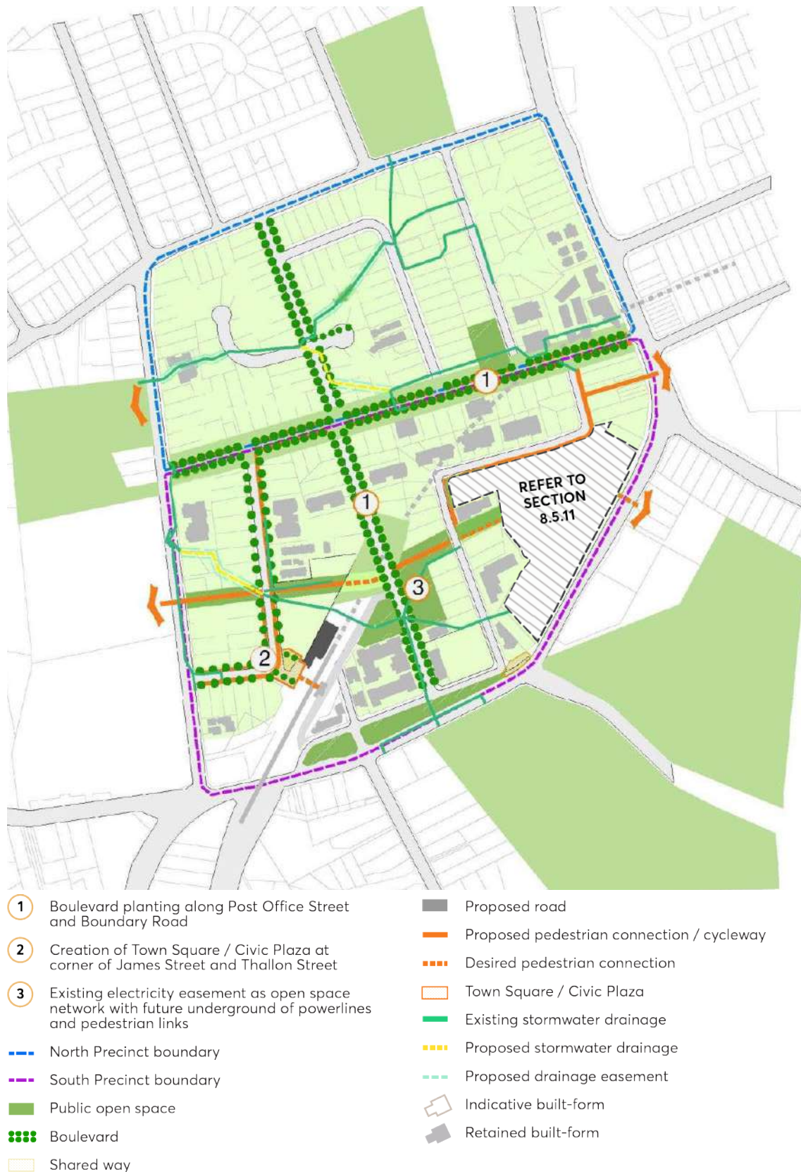
Figure 8.2.8.1.3.3 – Structure Plan – Public Domain
