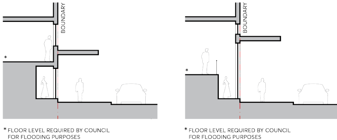
Figures 9.3.5.2.4 – Active Ground Floor: Floor level required greater than 1.5m above footpath level
