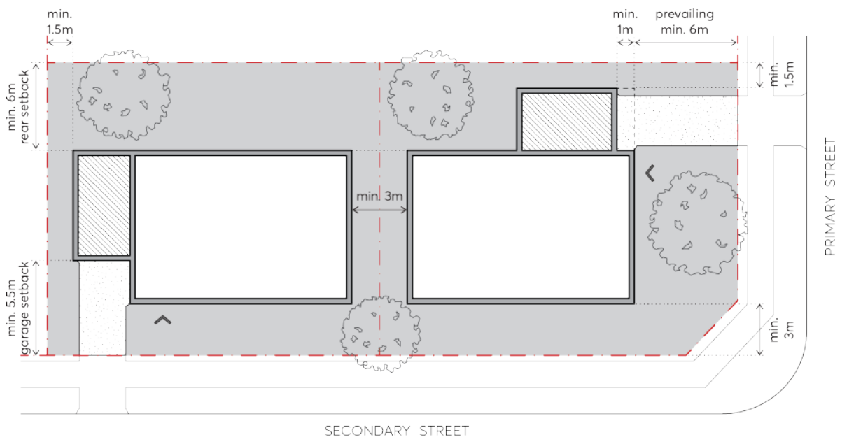
Figure 3.3.2.2.3 – Corner lot - detached dual occupancy site setbacks
