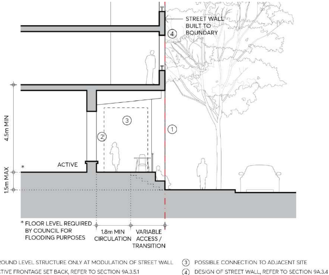
Figure 9.3.5.2.2 A – The Street Wall: Active frontage set back
