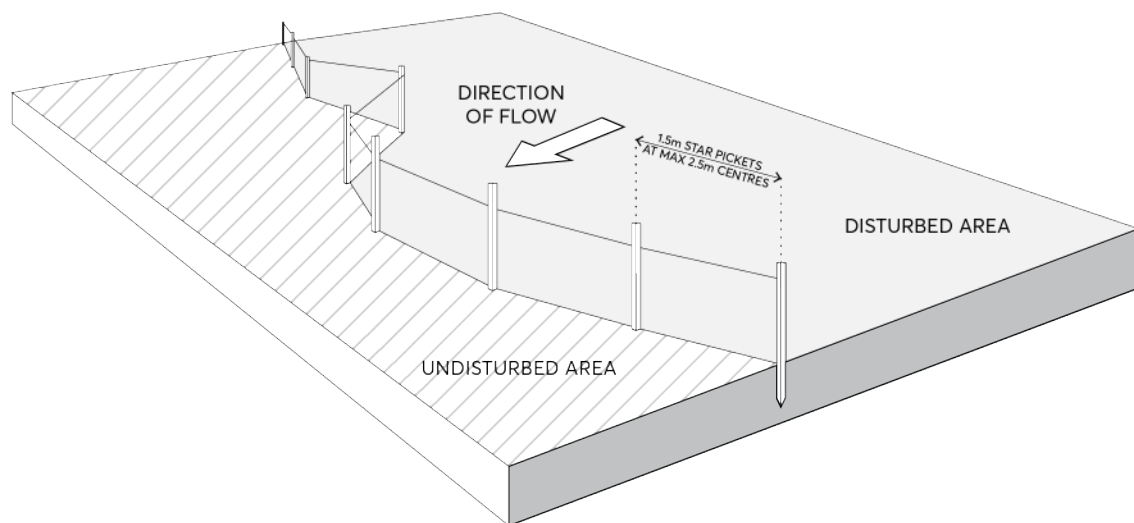
Figure 5.2.1.2 – Sedimentation Fencing (Source: Soils and Construction: Managing Urban Stormwater, Landcom, March 2004)
