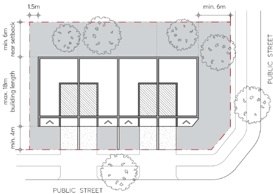
Figure 3.4.2.2.2 – Terrace Housing Corner Site Setbacks
