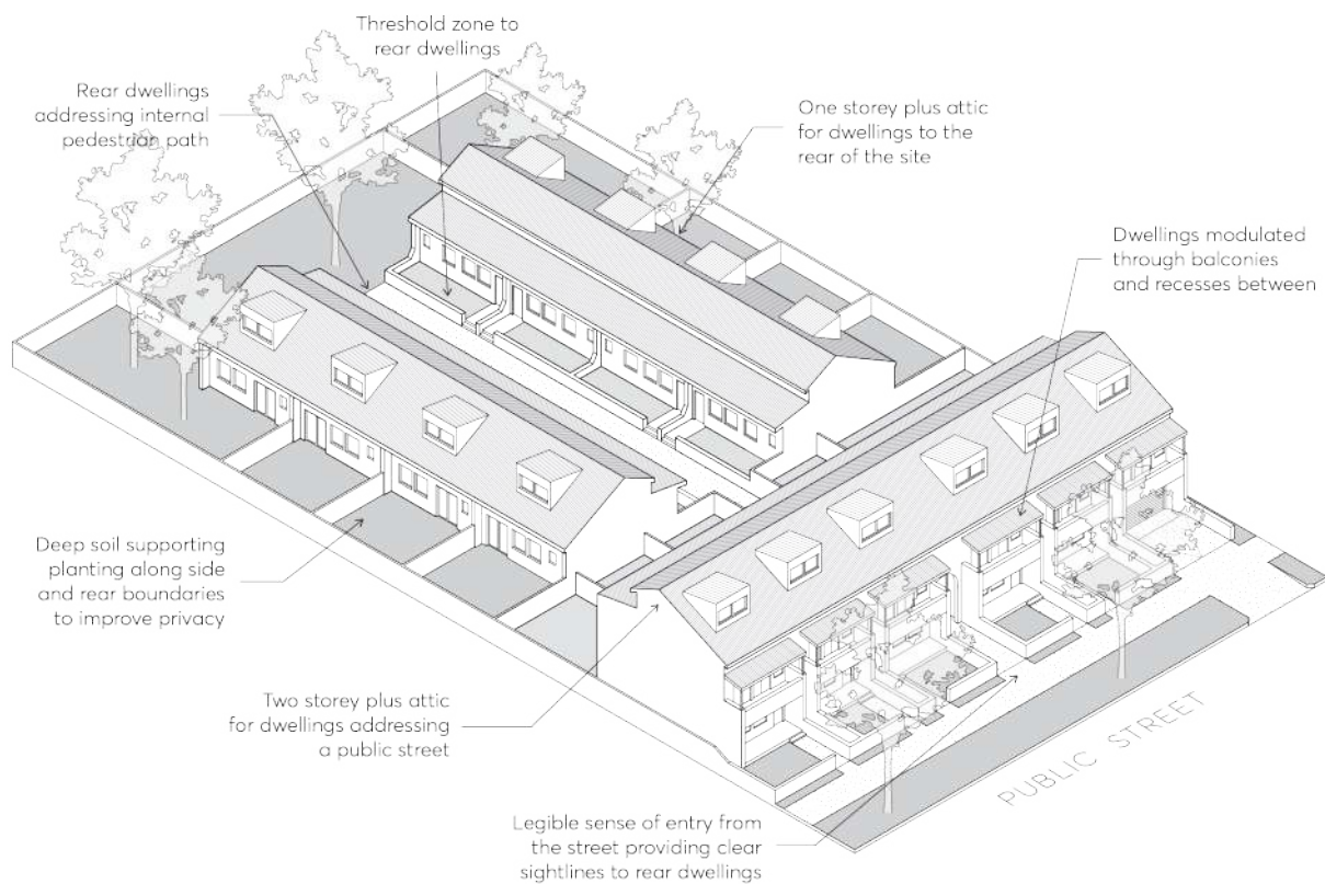
Figure 3.4.1.7.2 – T-configuration Townhouses
