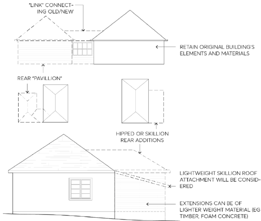
Figure 7.4.4 – Additions
