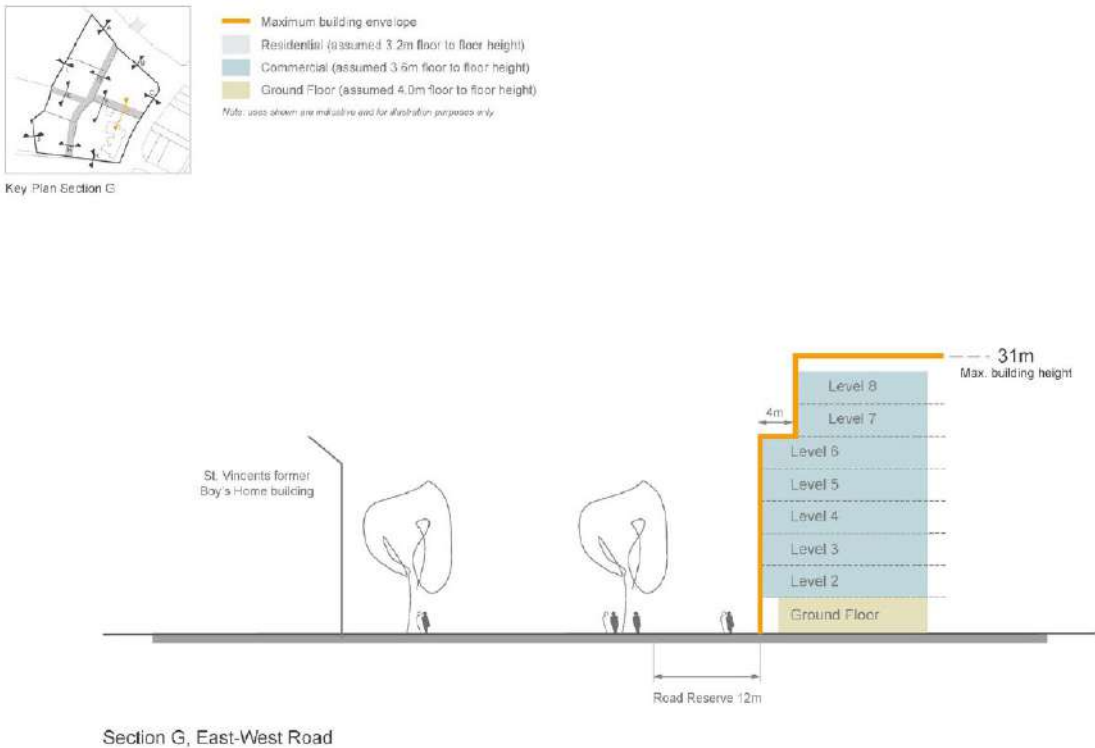
Figure 8.5.1.5.6 – Indicative Site Sections
