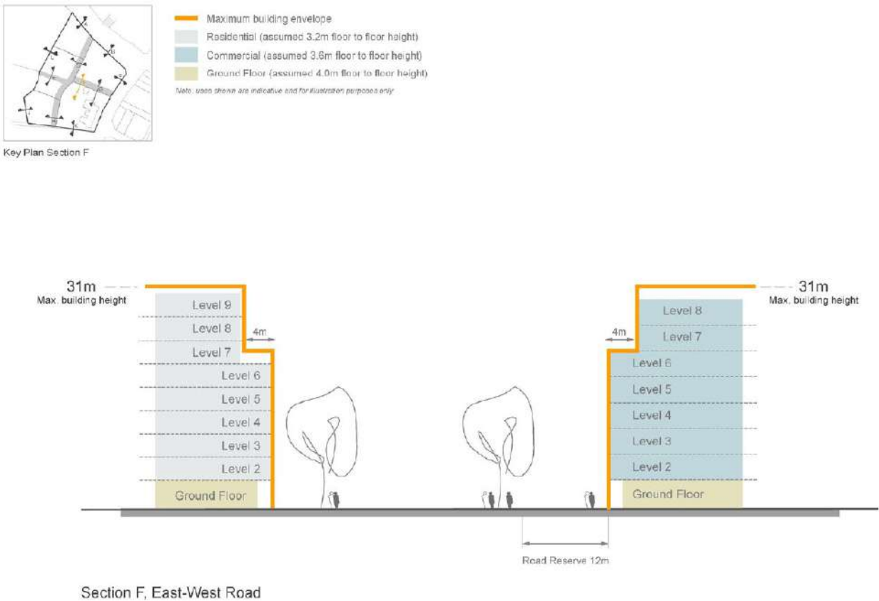
Figure 8.5.1.5.5 – Indicative Site Sections
