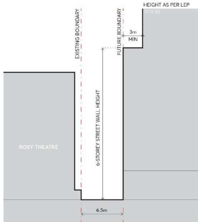
Figure 9.5.2.12 – New Laneway between the Roxy and Site 05 (Section F)
