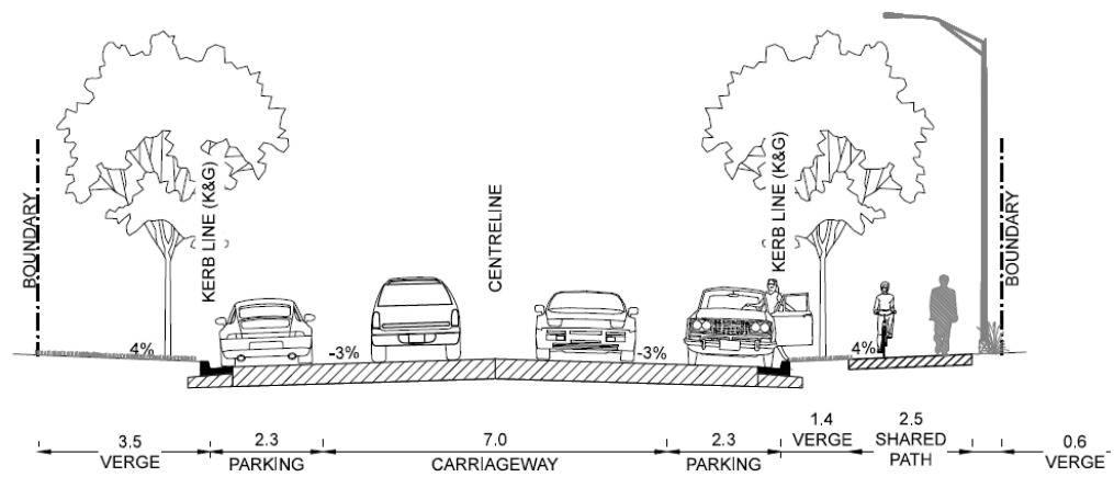
Typical Collector Road with Shared Path
